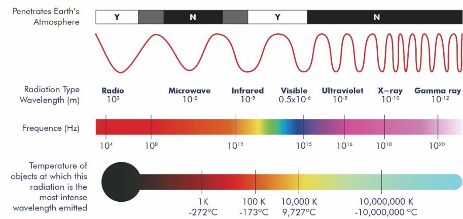
Illustration: The Electromagnetic Spectrum and the Temperature Spectrum, bottommost.
